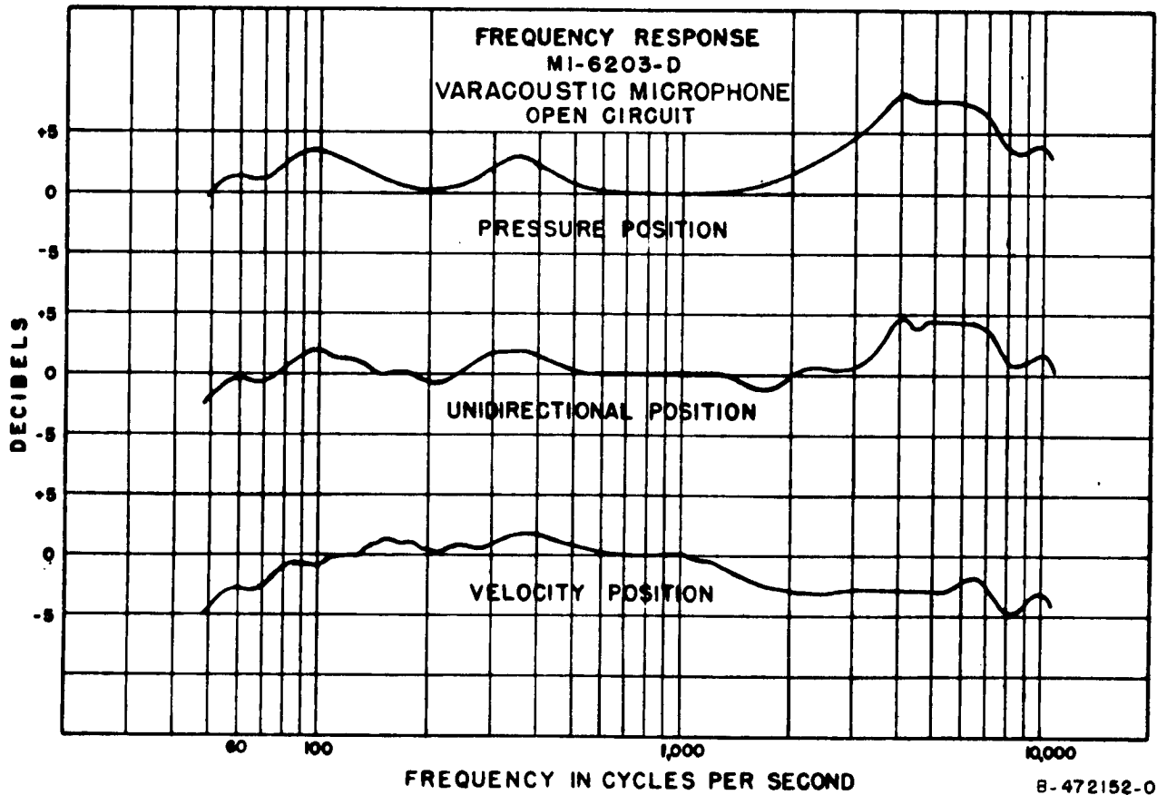
Figure 2 - Frequency Response
