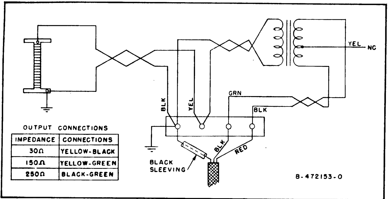
Figure 4 - Connection Diagram
