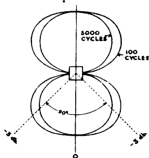
HORIZONTAL DIRECTIVITY OF VELOCITY MICROPHONE
