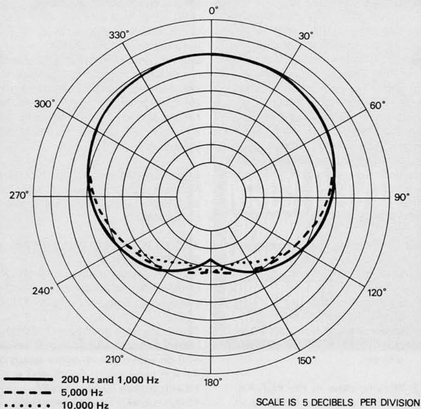
FIGURE 4 – Polar Response
