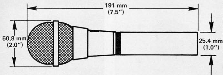
FIGURE 1 - Dimensions
