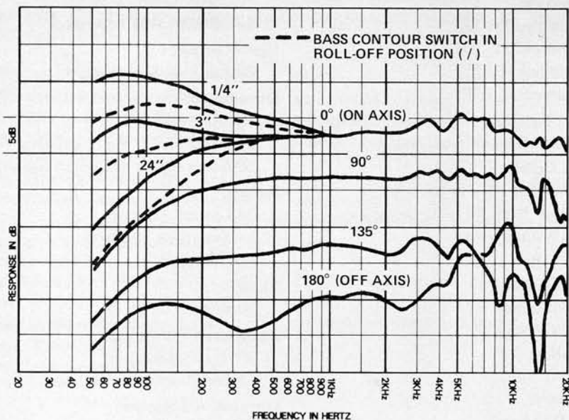
FIGURE 3 - Frequency Response
