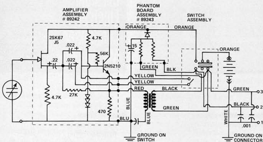
FIGURE 2 - Wiring Diagram
