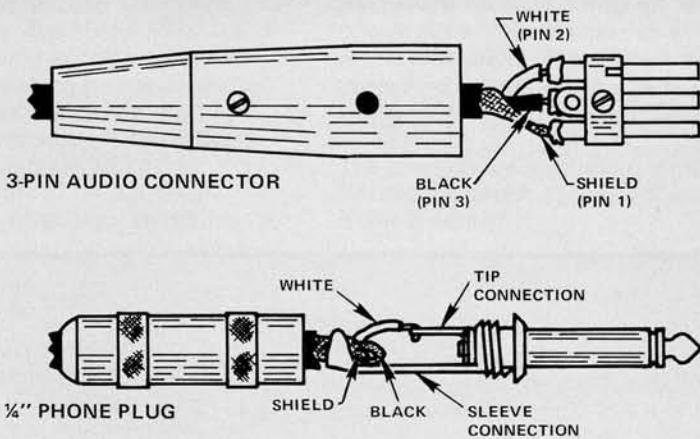
FIGURE 7 – 3-Pin Connector & 1/4" Phone Plug Wiring Connections
