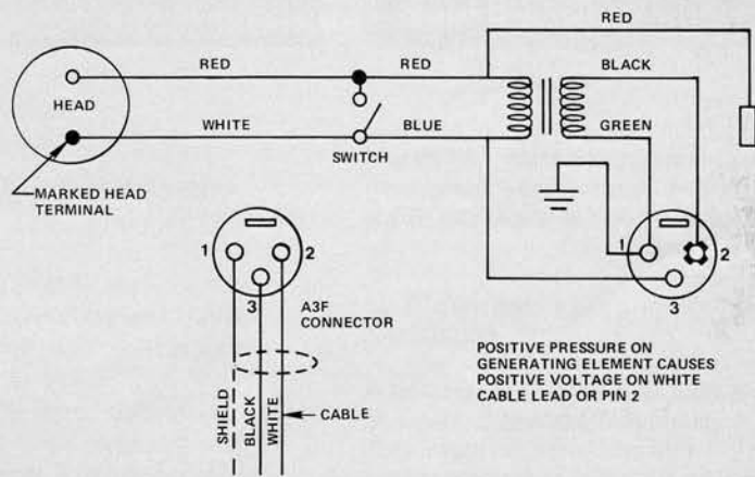
FIGURE 5—Wiring Diagram
