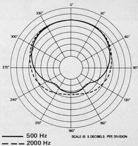
FIGURE 4 – Polar Response
